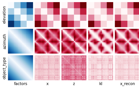
Figure 4: \beta -VAEs learn similar distances between observations at all levels of the network depending on the reconstruction loss. Rows: Different factors of the Cars3D dataset (Top to bottom: elevation, azimuth, car type), Columns: Distance matrices computed over factor traversals (Left to right: ground-truth distances, perceived distances between observations, \ell_2 distances over latent distribution means, KL divergences between latent distributions, perceived distances between reconstructions).
