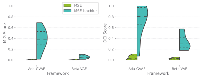
Figure 11: MIG and DCI scores for Ada-GVAE and \beta -VAE using the MSE loss and our modified loss function. Introducing a spatially aware loss function allows us to capture ground-truth distances between observations and allows the models to disentangle the adversarial XYsquares dataset.
