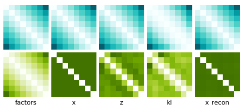
Figure 10: \beta -VAEs learn similar distances between observations. Top row: box blur augmented MSE. Bottom row: pixel-wise MSE loss. Columns: Distance matrices computed over factor traversals. All factors of XYsquares have the same statistics. This plot is constructed in a similar way to Figure 4.
