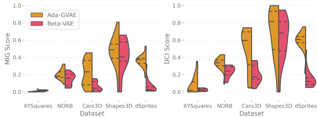
Figure 6: Densities over repeated runs for the attained MIG scores (left) and DCI Disentanglement scores (right) for the weakly-supervised Ada-GVAE (Left half of densities) and \beta -VAE (Right half of densities). XYSquares hurts the disentanglement performance significantly. Quartiles are marked with horizontal lines. We sweep over \beta values and latent dimension sizes. See our extended paper in Footnote 1 for details.
