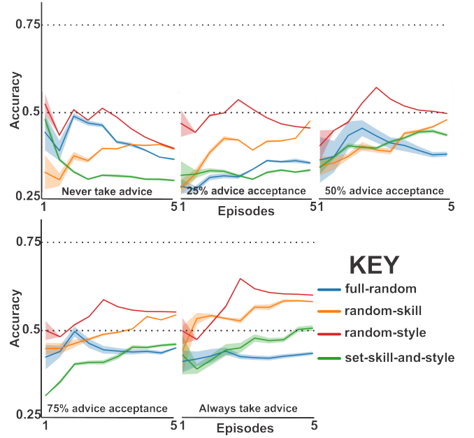
Figure 5: Comparison of the impact of a tailored advice generation pipeline on various advice acceptance thresholds and user archetypes for MiniDungeons domain.
