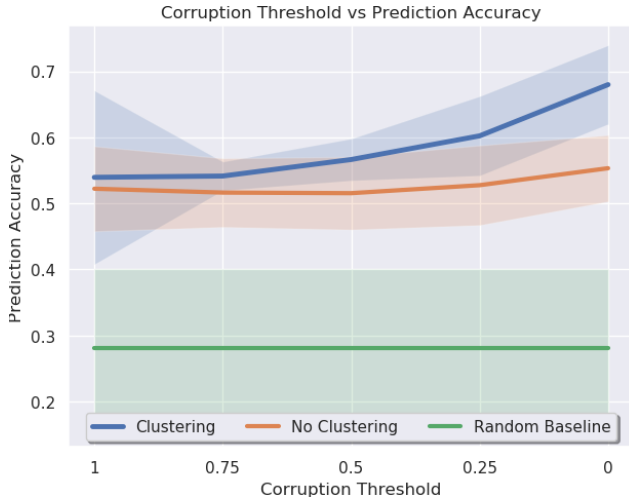
Figure 6: Comparison of the effect of differing the corruption threshold percentage on the models’ accuracy. Here “1” indicates random clustering and “0” perfect clustering
